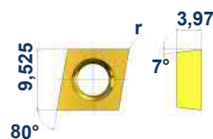
CC...09T3...
