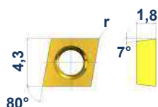
CC...0401...
