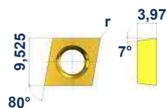
CC...09T3...
