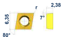
CC...0602...
