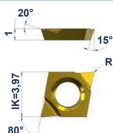
CDGT-0401...N
