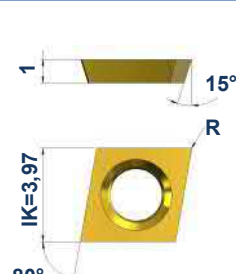
CDGW-0401...
