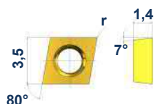
CC...0301...
